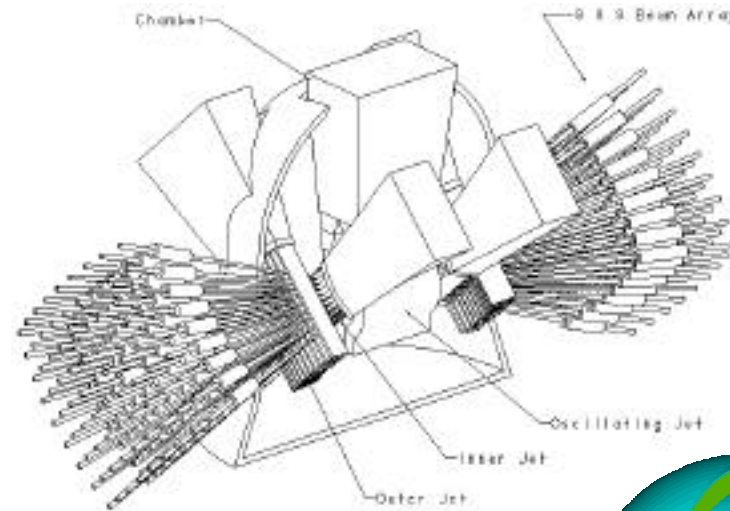
Pro-Engineer model of HYLIFE-II chamber and final focusing system
