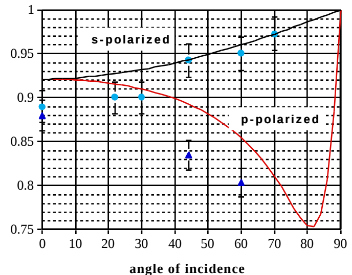
Comparison of thermopile reflectivity data with theoretical predictions for Al at 532 nm
