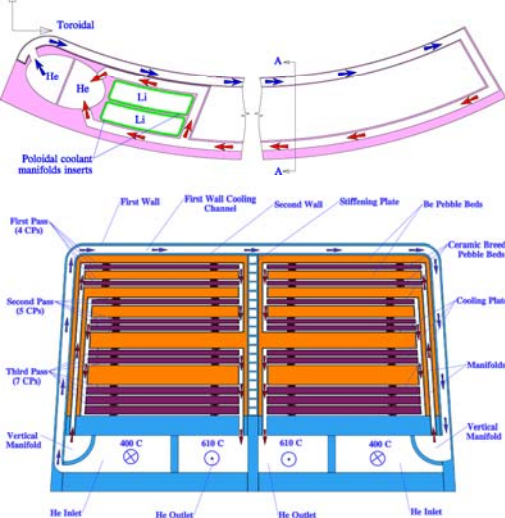
Flow Channel Inserts in the Poloidal Li-Manifolds(Half Period)
