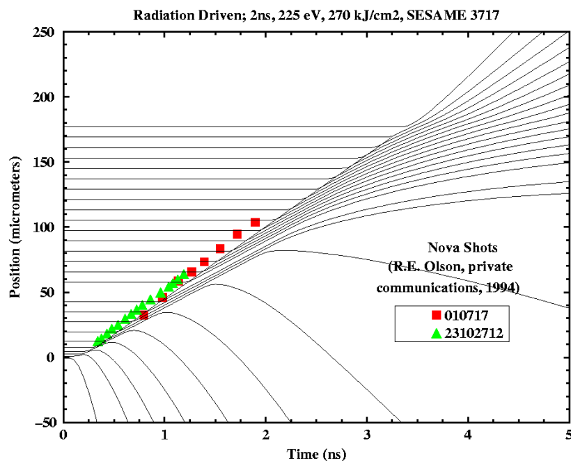
BUCKY Simulation of Shock in Aluminum
