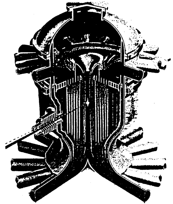
HYLIFE (1985)
