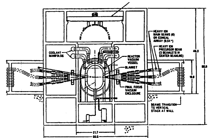
PROMETHEUS-H (1992)
