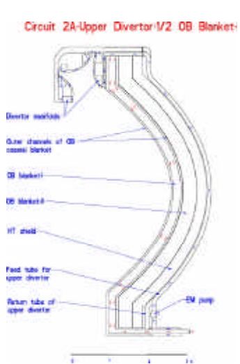
Figure 2. Upper Divertor + 1/2 OB Blanket
