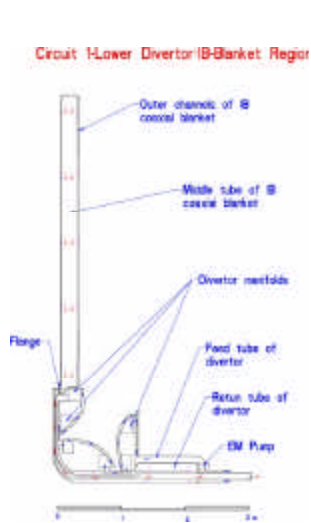
Figure 1. Circuit 1 – Lower Divertor and IB Blanket
