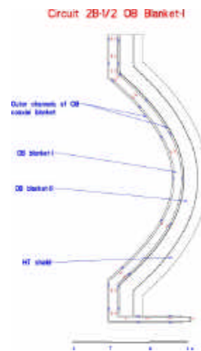
Figure 3. Half OB Blanket
