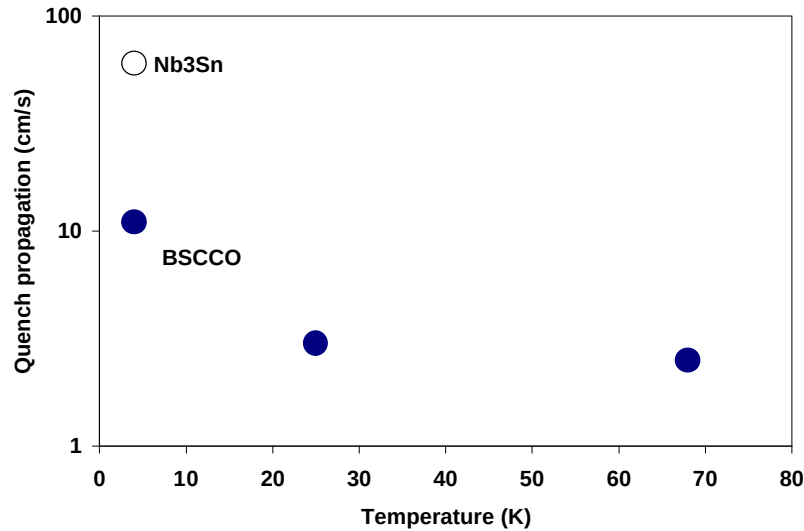
Figure 4. Quench propagation speed in LTS and HTS (2212 BSCCO).
