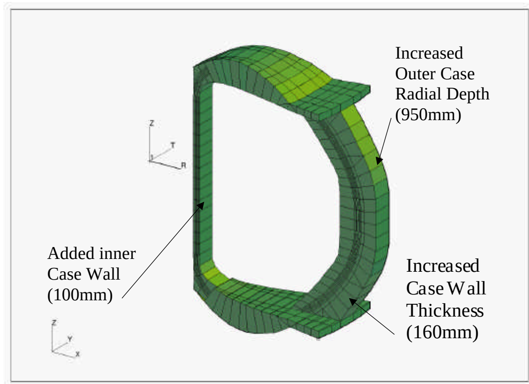
Figure 13. Aries-AT TF Coil/Case FEA Model With Reinforced Walls
