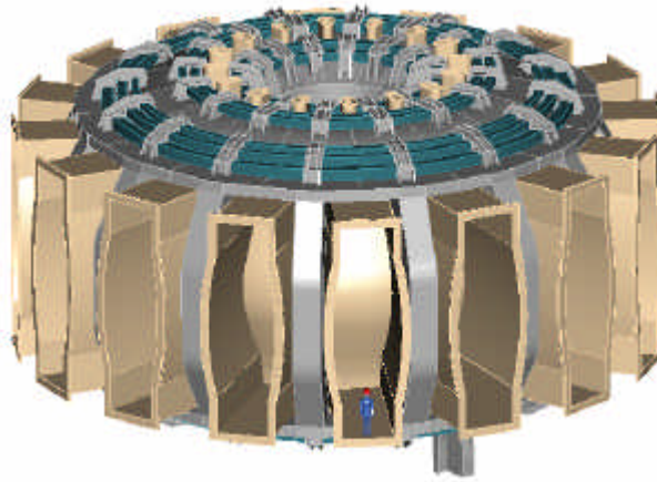
Figure 7. Aries-AT General Arrangement
