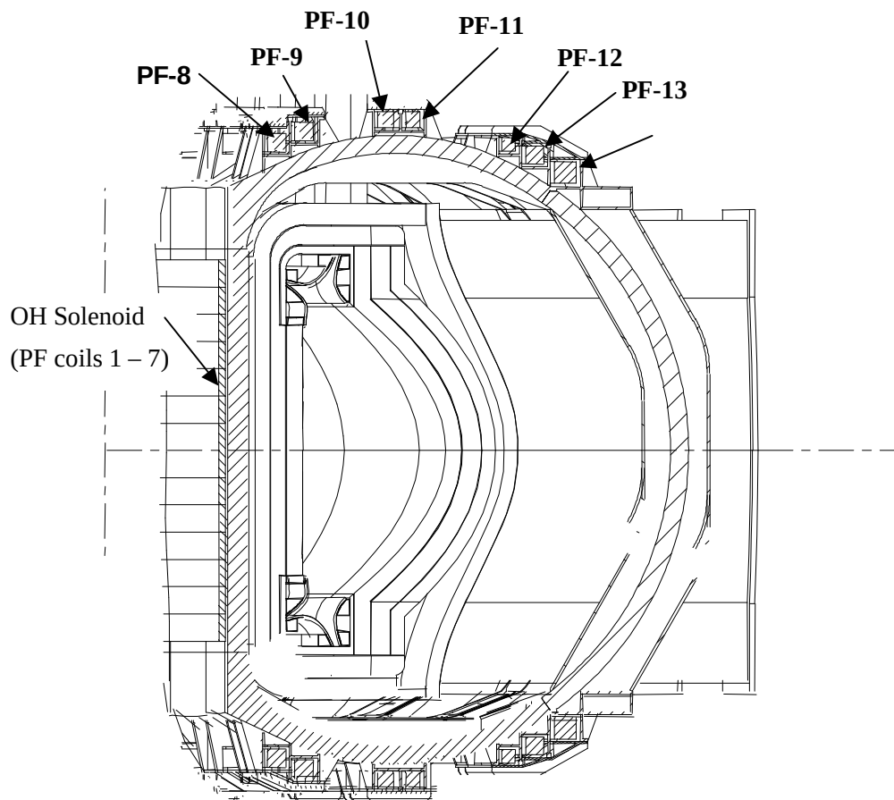
Figure 20. PF Coil Locations
