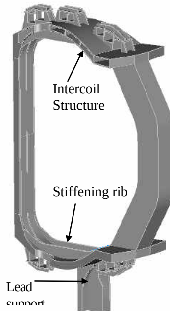
Figure 11. TF coil
