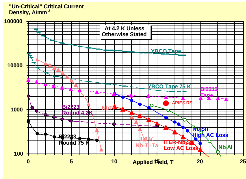
Figure 1. Critical current density for several HTS and LTS materials as a function of the applied field, for either liquid nitrogen temperature or 4 K (if not indicated).
