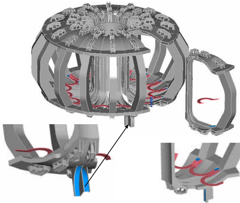
Figure 12. Full TF coil assembly and local lead details
