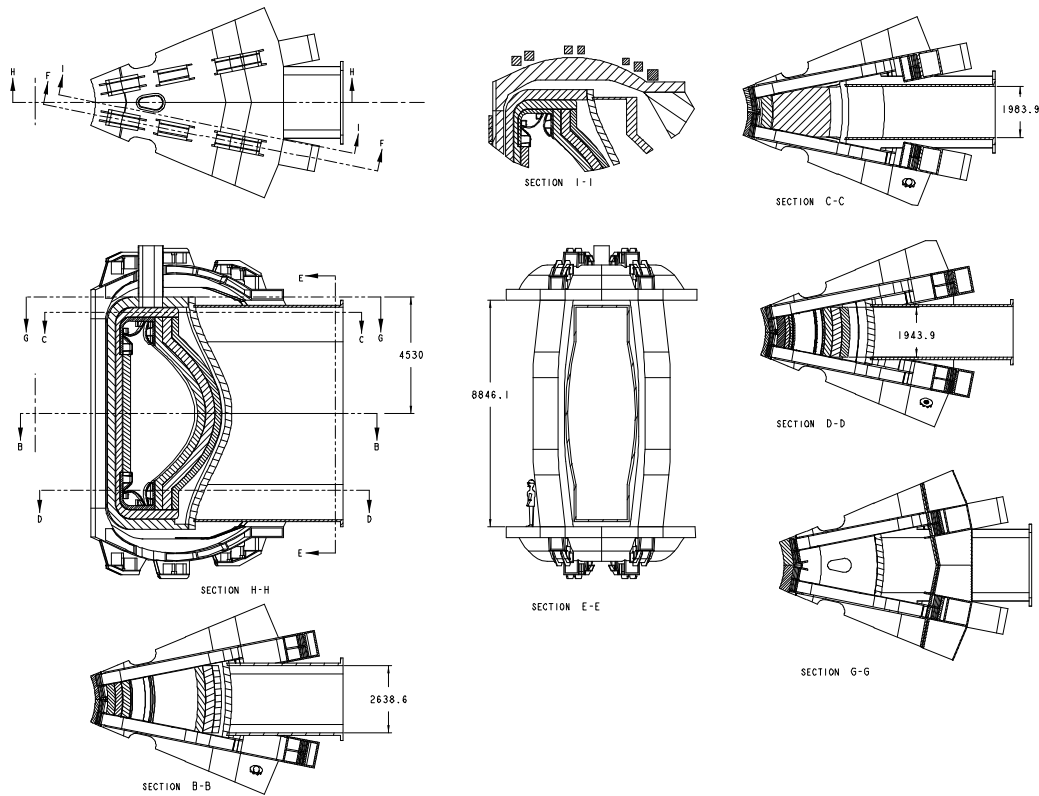
Figure 9. TF/VV Sector Geometry Details
