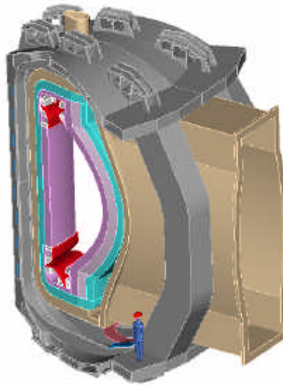
Figure 8. TF/VV sector
