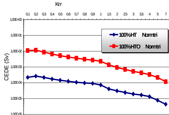
Figure 3.- Effective dose equivalent vs. distance for HT and HTO in normal conditions [7].
