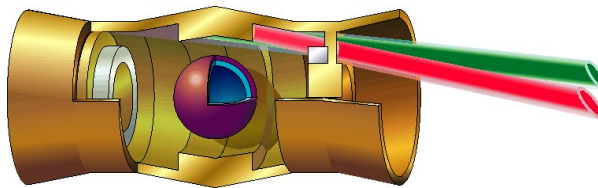
FIG. 2. Close-coupled, heavy-ion indirect drive target concept for IFE designed at LLNL. The length of the target is 20 mm and the average radius is \sim 5 \text{ mm} . The central fuel capsule is \sim 4.7 \text{ mm} in diameter and consists of a 0.2 mm thick bromine doped beryllium ablator followed by a solid DT fuel layer of 0.32 mm thickness.
