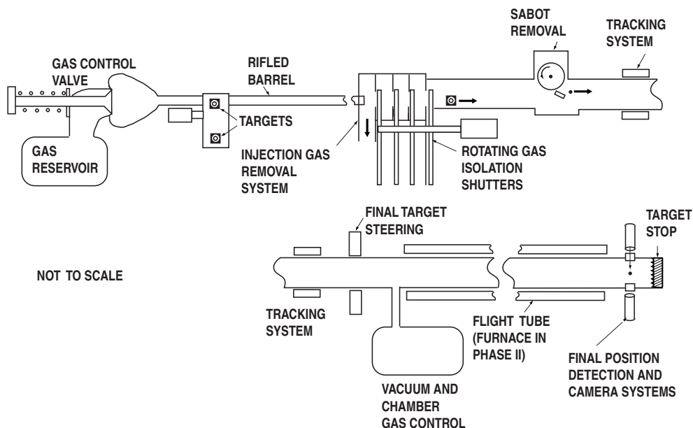
FIG. 6. Overview of experimental target injection and tracking facility.
