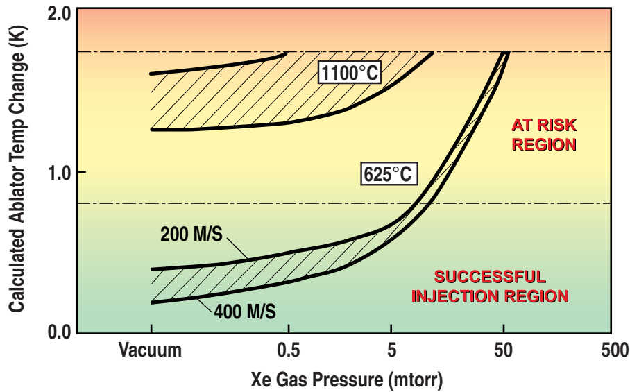
FIG. 5. Calculated outer DT ablator temperature following injection. A temperature <18.8 K is considered to be successful injection; T > 19.8 K is excessive heating during injection.
