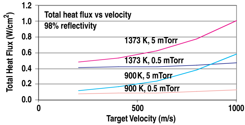
FIG. 3. Average total heat flux on a target moving through a xenon-filled reaction chamber.
