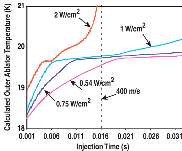
FIG. 4. Finite element results showing the temperature rise in the outer DT ablator as a function of uniformly distributed surface heat flux and injection time (time in the target chamber).
