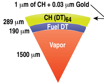
FIG. 1. Direct drive target concept for IFE designed at NRL.
